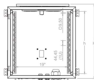
Inside view
