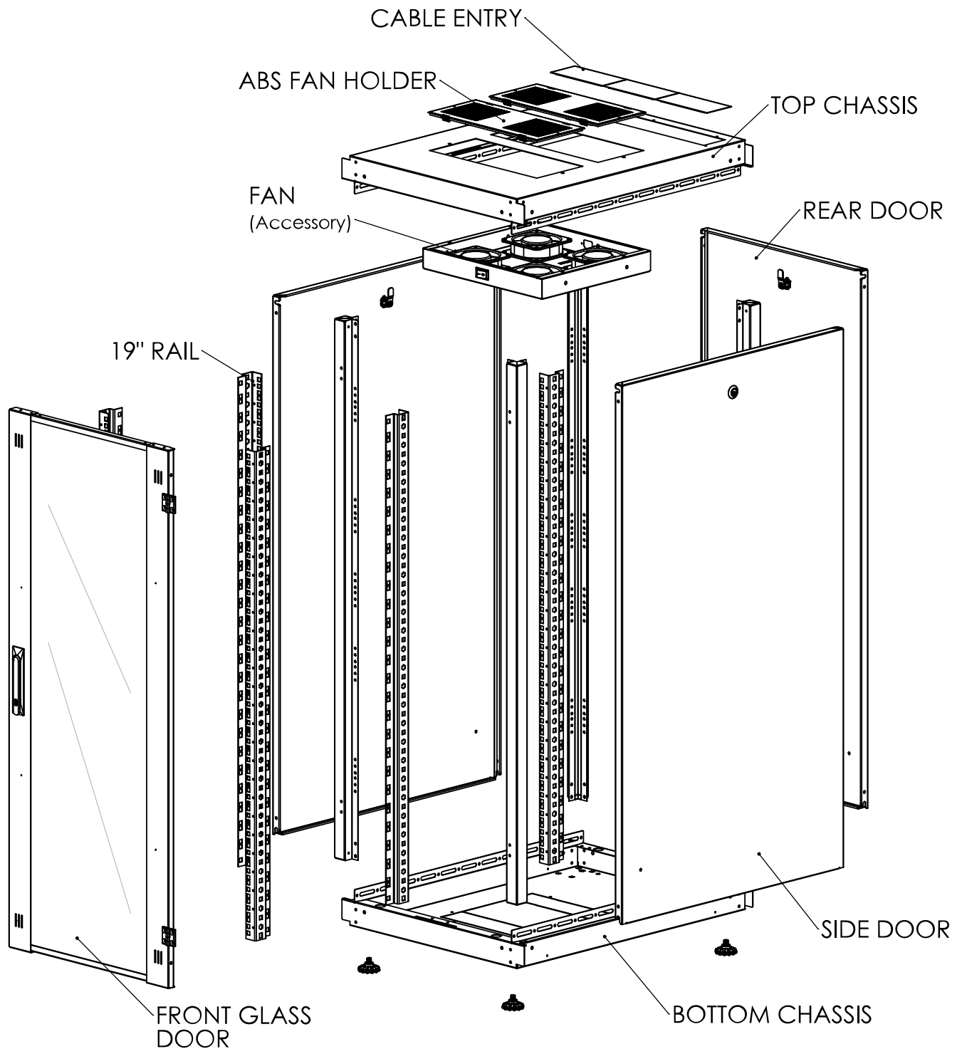
Exploded view
